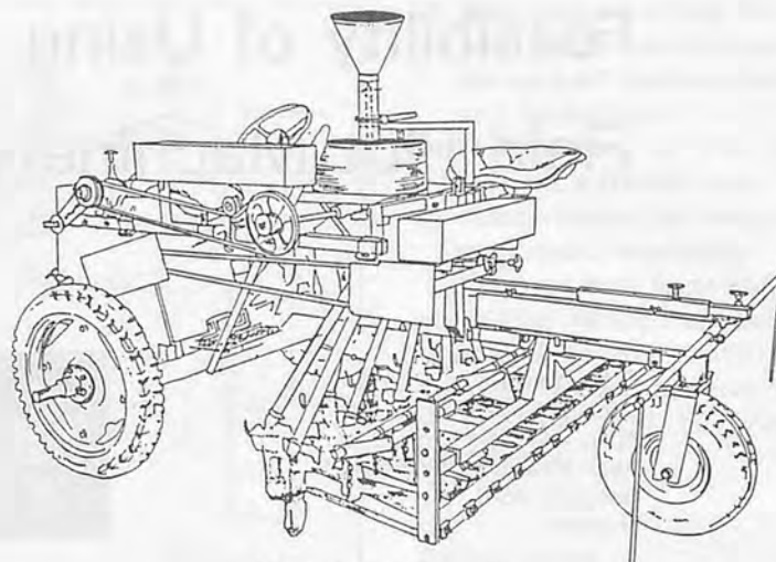
Fig. 1 Oyjord plot drill.
