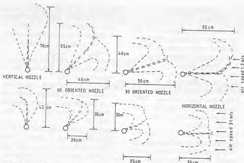
Fig. 4 Fog formation pattern as affected by nozzle orientation and air speed.
