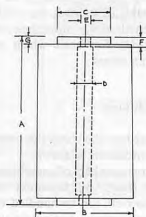
Fig. 1 Dimension of filter element.
