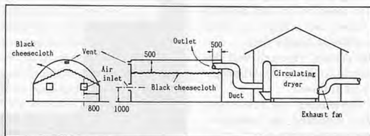
Fig. 3 Artificial drying facilities by the solar energy.
