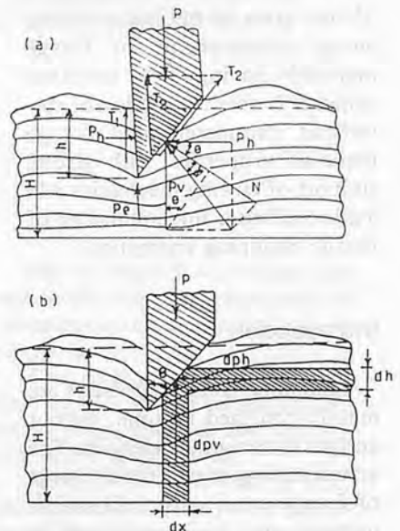
Fig. 2 Force relations for a knife penetrating into the plant material.
