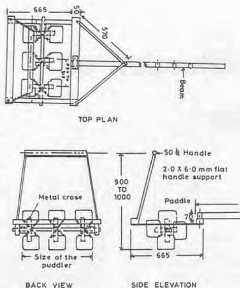
Fig. 1 Rotary blade bullock-drawn puddler.
