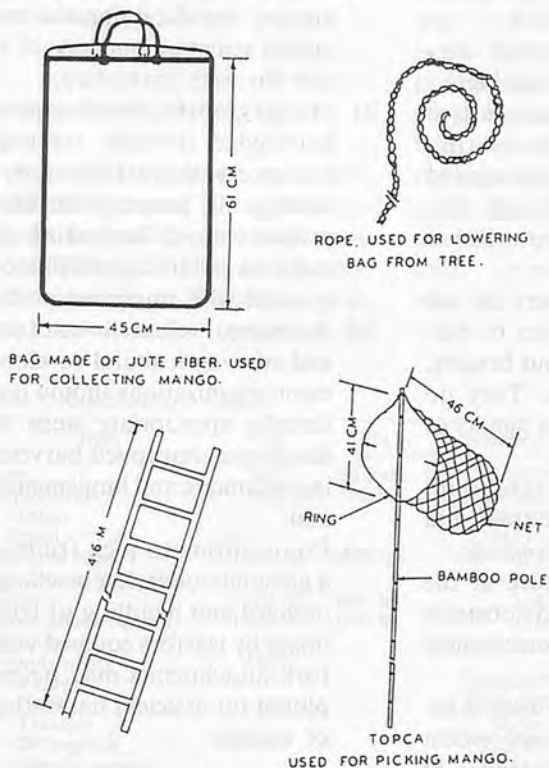
Fig. 6 Equipment used in existing practices of harvesting.
