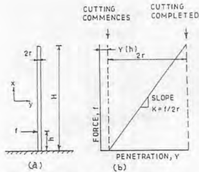
Fig. 4 a) Model of the forage system as a uniform cantilever subjected to a forcing function, f . b) Model of the forcing function, f as it penetrates and cuts the stem.
