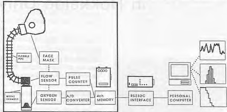
Fig. 9 Portable energy expenditure measuring apparatus.
