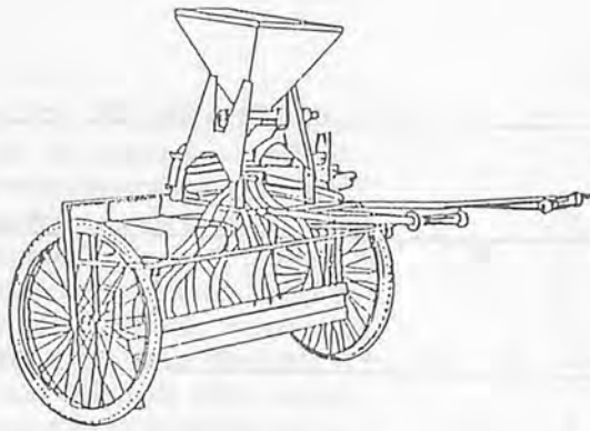
Fig. 3 Fertilizer distributor, Hege-33.
