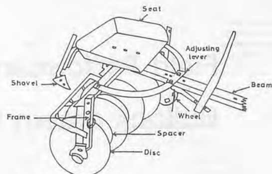
Fig. 2 Bullock-drawn harrow-cum-puddler.
