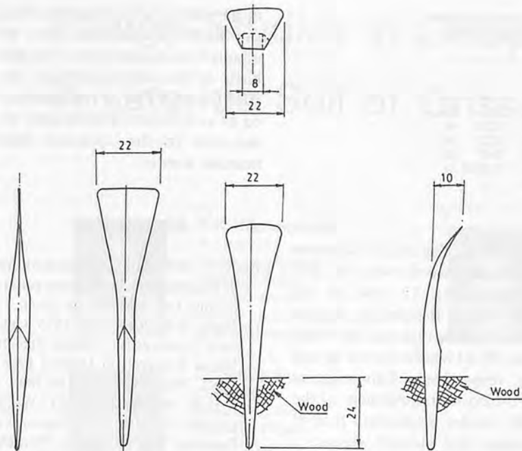
Fig. 4 Spike before bending, a) side view, b) front view.
