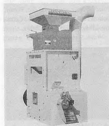
YANMAR Rice Huller/Polisher Mill Mate YHP800. This machine is a complete direct-through rice mill consisting of a hulling section winnower and polishing section. Capacity in paddy 800-900kg/h. Required power: 15-18HP.
