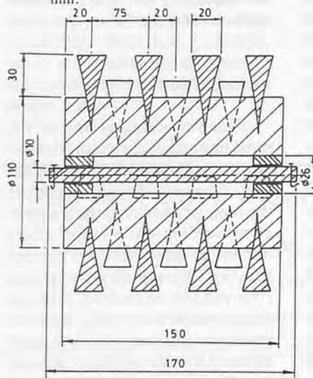
Fig. 2 Longitudinal section of wooden core.
