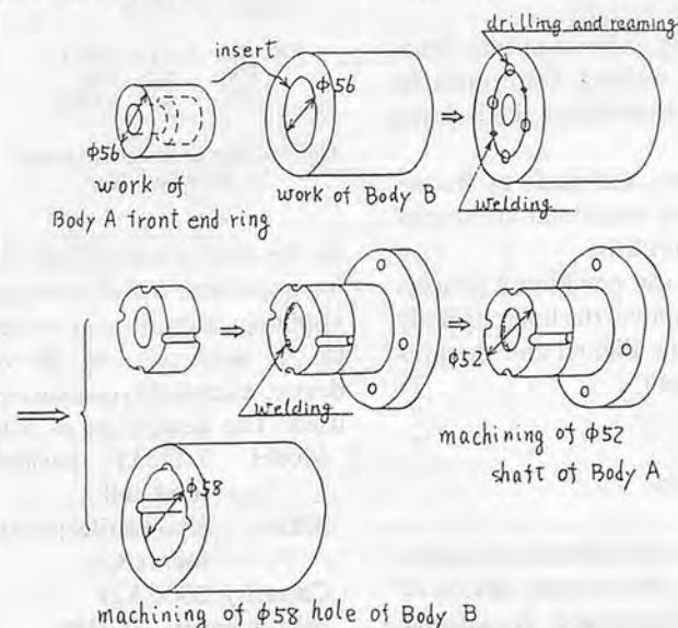
Fig. 6 Manufacturing process of Body A and B.
