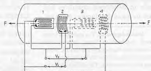
Fig. 4 Layout of strain.
