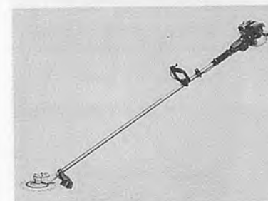
KOMATSU ZENOAH Reciprocator SGC220DL. Engine: 22.5cc, Dry weight: 6.5kg, Cutting Blade: 230mm, 20-toothed, heat-treated steel blade.
