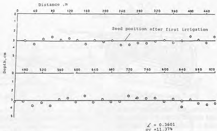
Fig. 6 Vertical placement of wheat seed by Oyjord drill.
