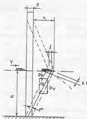
Fig. 3 Free cutting of standing forage materials.
