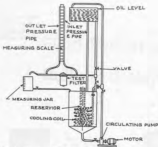
Fig. 2 Test set-up for flow rate and pressure drop.
