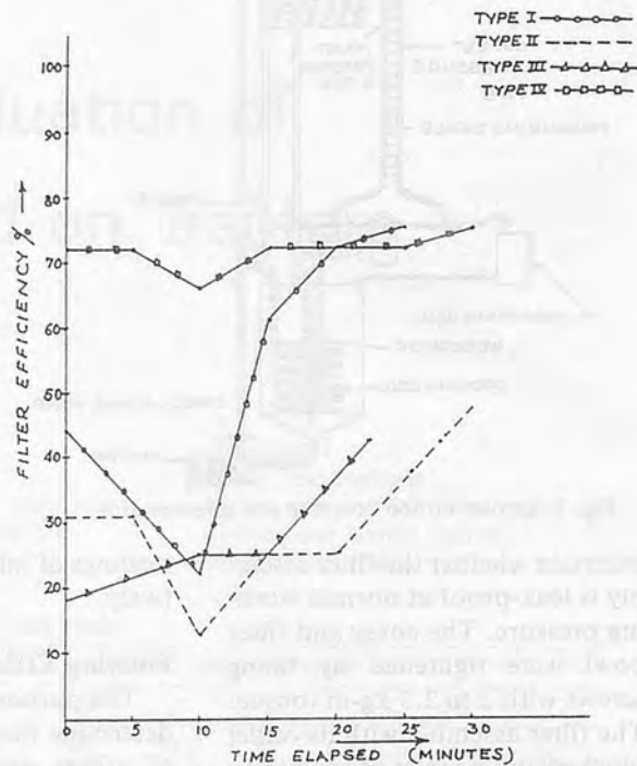
Fig. 5 Filtering efficiency of pre-filter.
