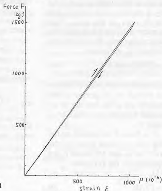
Fig. 10 Calibration graph.
