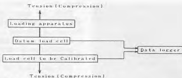
Fig. 7 Calibration system.
