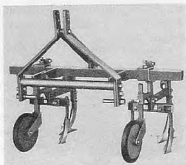
SUKIGARA Double Row Cultivator Model TBC. The row width can be controlled easily and quickly by adjusting each bolt at the left and right of tool bar. Row width: 600-900mm. Suitable working speed: 3-5km/h. Power required: 11-20HP.
