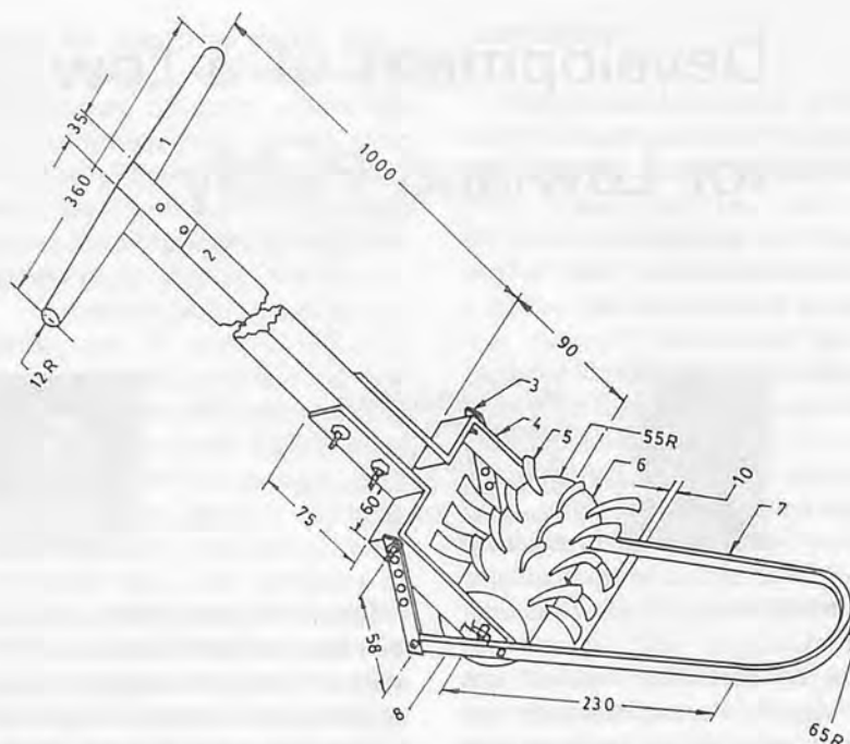
Fig. 1 Push type weeder showing components: 1—Grip, 2—Handle, 3—Gauge bar, 4—Frame, 5—spike, 6—150mm long wooden core, 7—Skid-frame, 8—Axle. Unit: mm.
