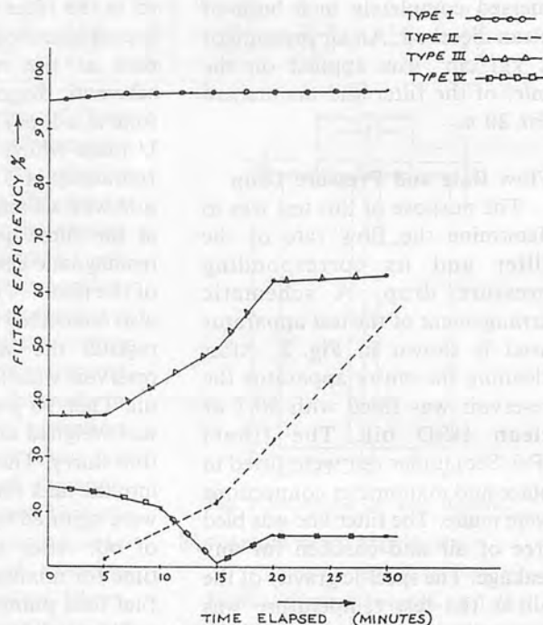
Fig. 6 Filtering efficiency of fine filter.
