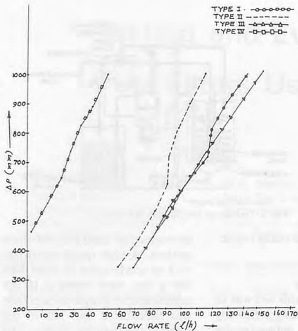
Fig. 4 Pressure drop vs flow rate test rated flow at 1 m head.
