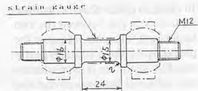
Fig. 5 Strain bar.
