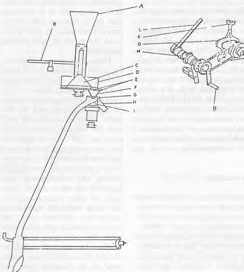
Fig. 2 Seed metering system on Oyjord plot drill.
