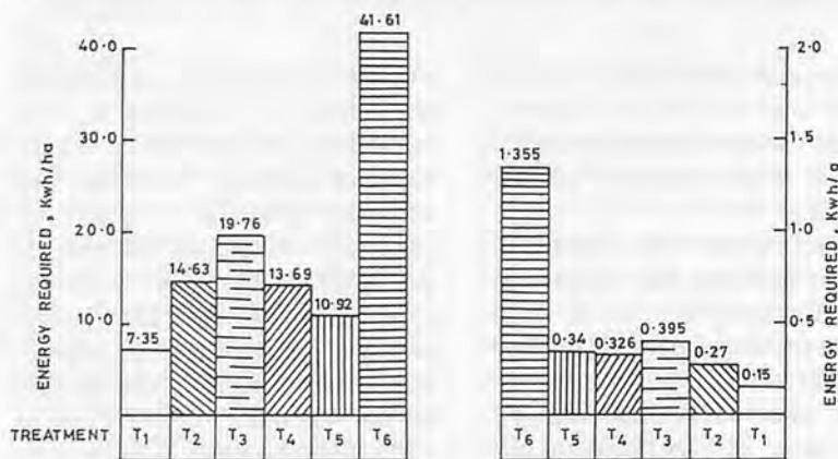
Fig. 4 Energy requirements influenced by puddling treatments.
