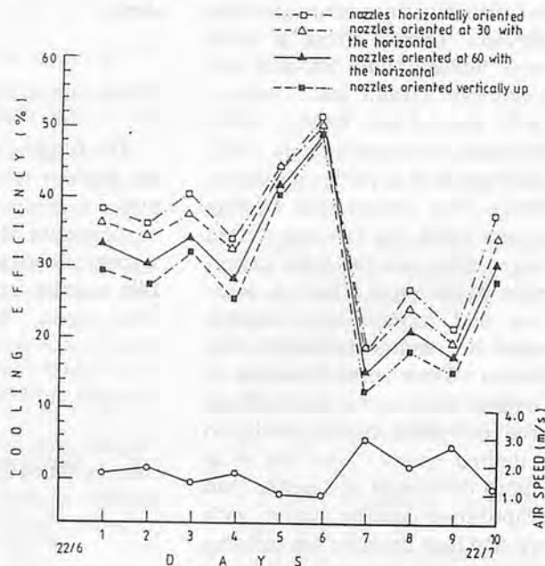
Fig. 3 Cooling efficiency of foggers as affected by nozzle orientation and air velocity.
