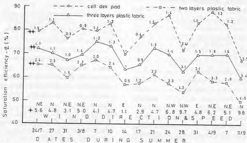
Fig. 5 Saturation efficiency ( \eta ) of the three types of wetted pads used in the experimental work. * wind velocity, m/s and ** air speed through pad, m/s.
