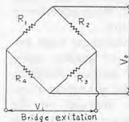
Fig. 3 Wheatstone bridge circuit.
