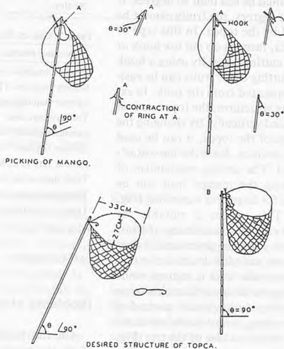
Fig. 7 Mechanism of mango picking by topca.
