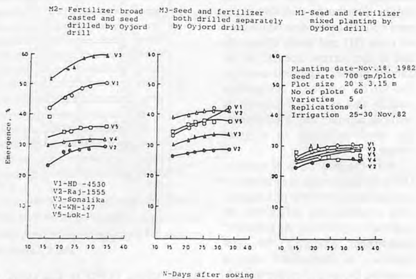
Fig. 7 Effect of planting method on seed emergence by Oyjord drill on wheat.
