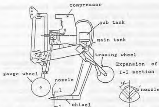
Fig. 4 Side view of soil loosening machine with compressed airblast.
