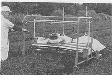
MATSUMOTO Tea Harvester MST-E2. Simple and easy operation. Self-propelling; Labor-saving. Picks best quality leaves with high efficiency.
