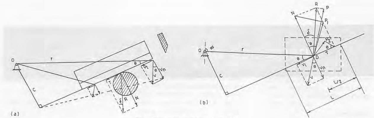
Fig. 1 Kinematic relations in cutting.
