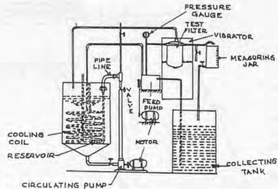
Fig. 3 Test set-up for filtering efficiency.
